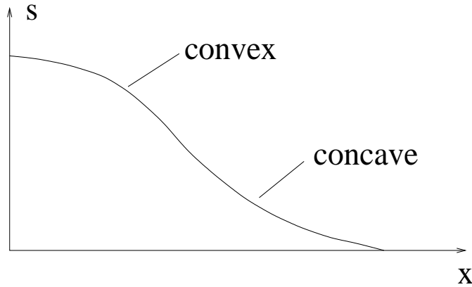
Figure 4: Convexity and concavity.
