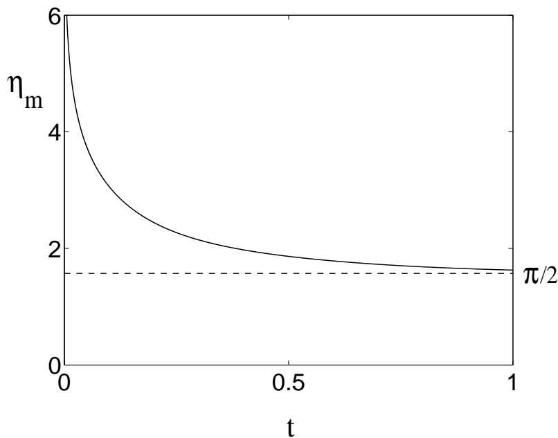
Figure 7: Evolution of the front position \eta_m as a function of t , for the solution in figure 6. The singularity at t = 0 is approximately (numerically) logarithmic.
