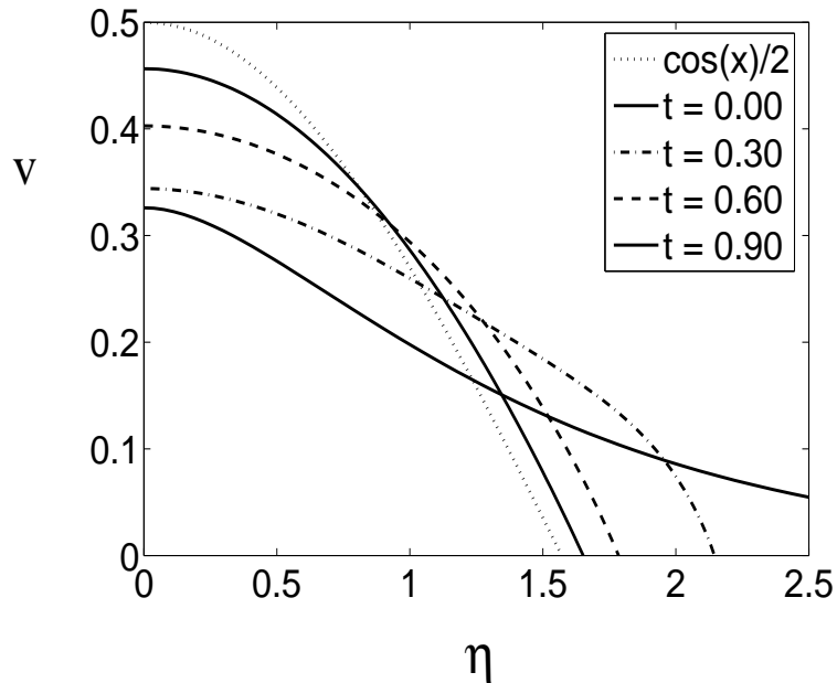
Figure 6: Relaxation of the solution of (5.19) to the steady state. The initial condition v_0(\eta) (using the formulation in (5.25)–(5.27)) is given by v_0 \propto \exp\left\{-\frac{\eta^2}{\eta+1}\right\} .
