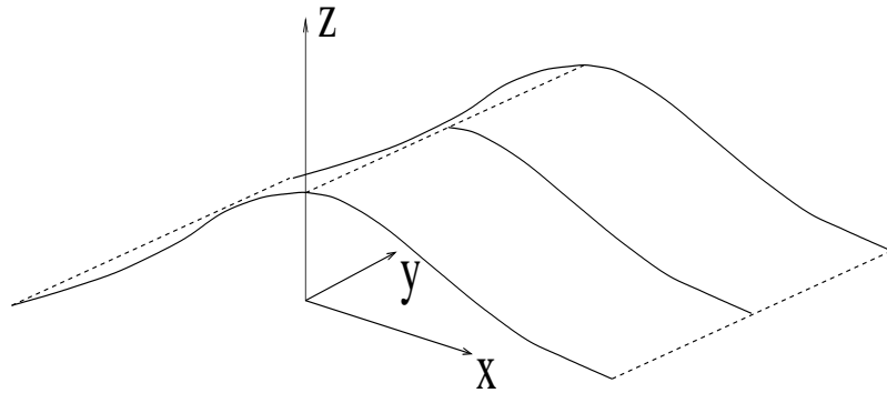
Figure 3: One-dimensional hillslope geometry.
