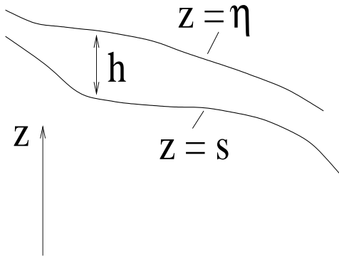
Figure 2: Geometry of overland flow.
