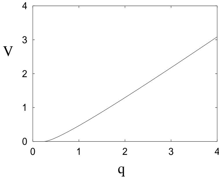
Figure 5: V(q, S) given by (3.10) for \beta = 0.1 , \tau_c^* = 0.5 .
